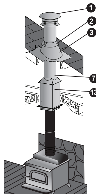
Single-Story Woodstove
