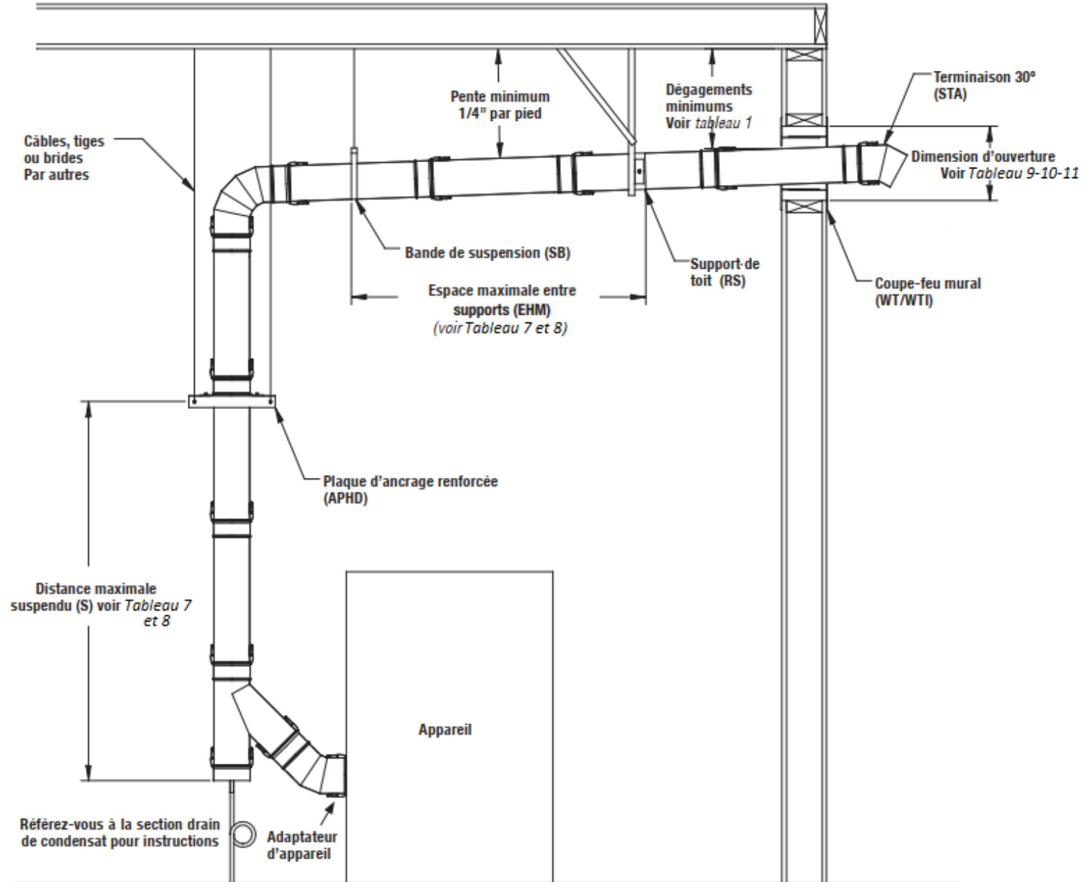
Figure 5- Installation horizontale
