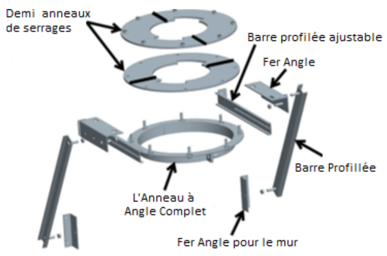
Figure 54a: Support mural (WSHD)
