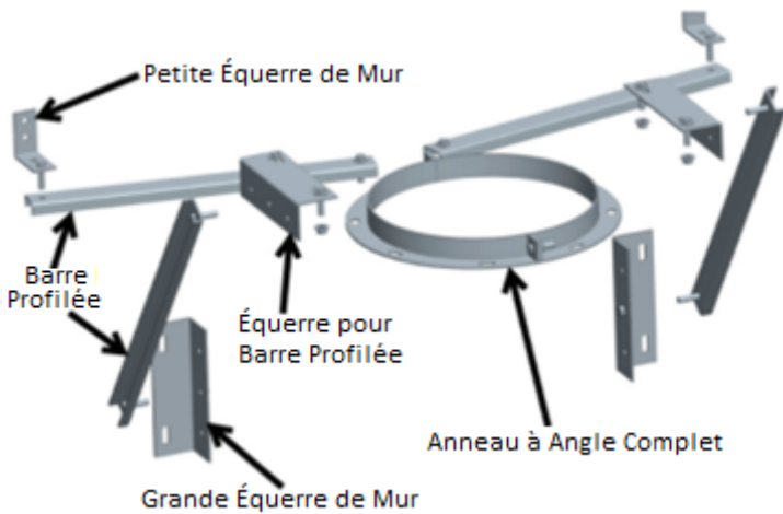
Figure 55: - Guide mural robuste (WGHD)
