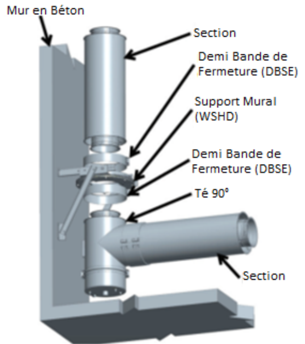
Figure 44: - Support de départ suspendu
