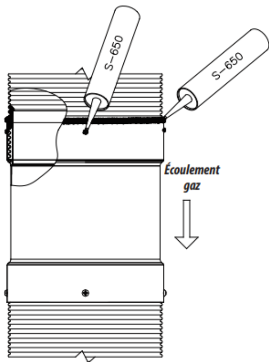
Figure 23 - Scellant Seal Flex Flex S-650
