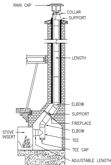
Fig. 9 - Existing fireplace relining installation
