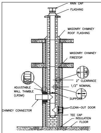
Fig. 4 - New masonry liner installation for interior chimney
