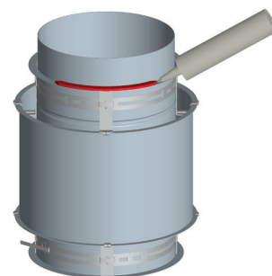
Figure 7 - Joint Assembly Step 2
