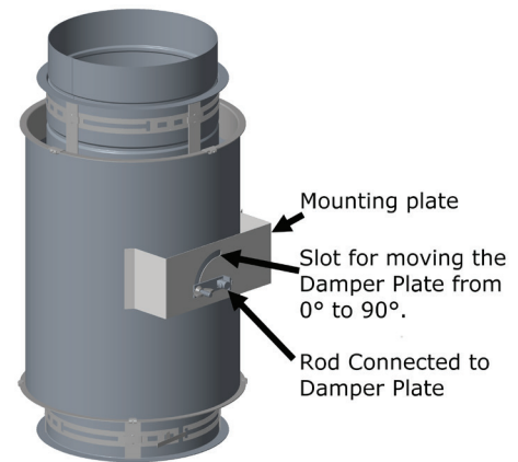
Figure 81a - Damper
