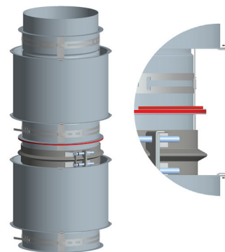
Figure 8 - Joint Assembly Step 3
