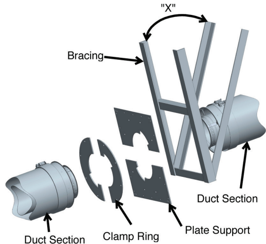
Figure 42 - Anchor Plate Horizontal Bracing
