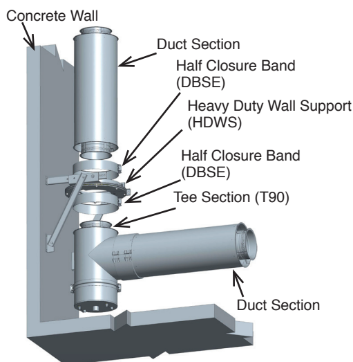
Figure 104: Suspended Tee Support
