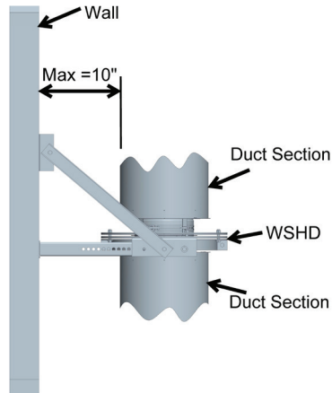
Figure 47c - Maximum Adjustment
