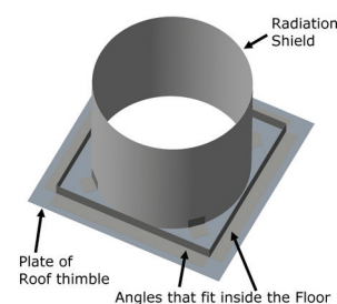
Figure 58a - Roof Thimble (RT)
