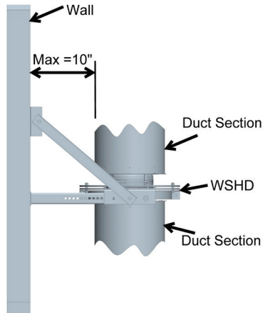
Figure 47c - Maximum Adjustment
